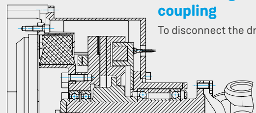
Type AC...F2 with electromagnetic coupling
