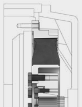
Type AC...F2 with splined taper bush
