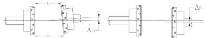
Angular Misalignment
